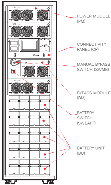
MPW 130 CBC Combo Cabinet MPW 42-126 kW (fronte)
